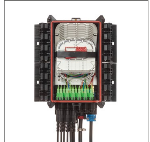
BPEO S1.5 ECAM Connect with DualDrop cable
