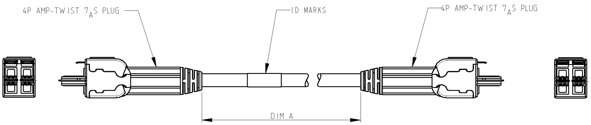
DRAWING SCHEMATIC
