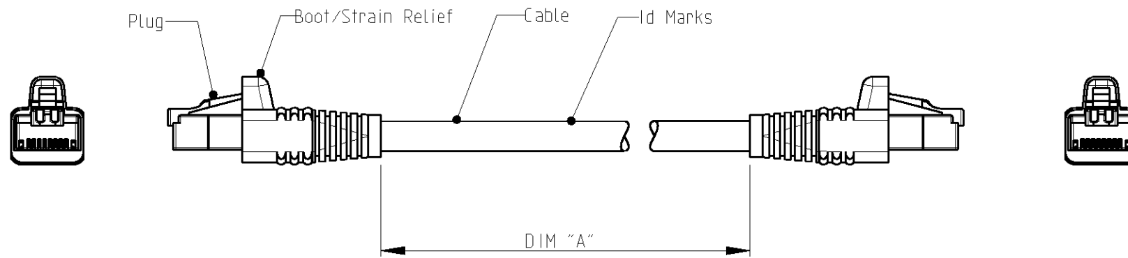
SCHEMATIC VIEW
